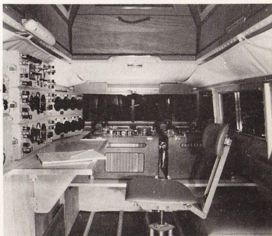
THE CARAWAGON is capable of being modified for an almost endless variety of purposes. The examples shown here are from the fleet of B.B.C. Outside Broadcast Vehicles.
